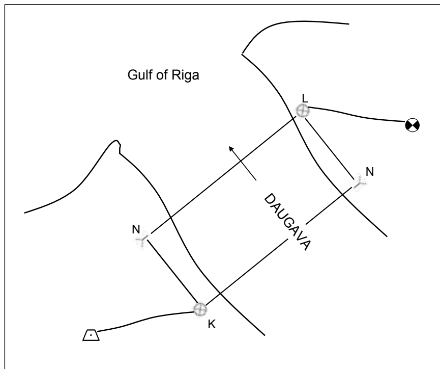
Figure 4. The scheme of levelling across the Daugava at the creek.
